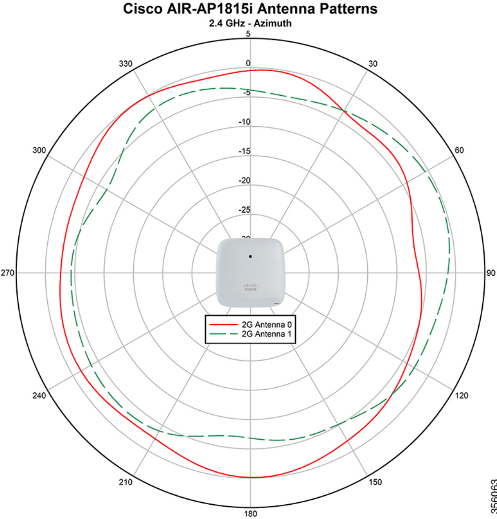
Figure 2 2.4 GHz - Azimuth Radiation Pattern
