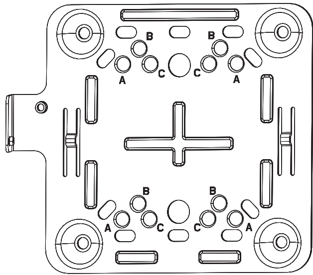
Figure 7 AIR-AP-BRACKET-8
