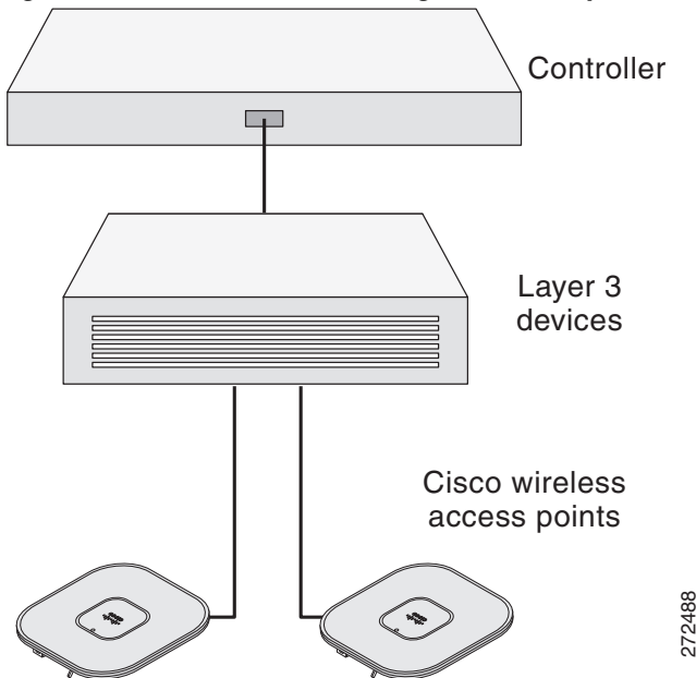
Figure 8 Pre-Installation Configuration Setup
