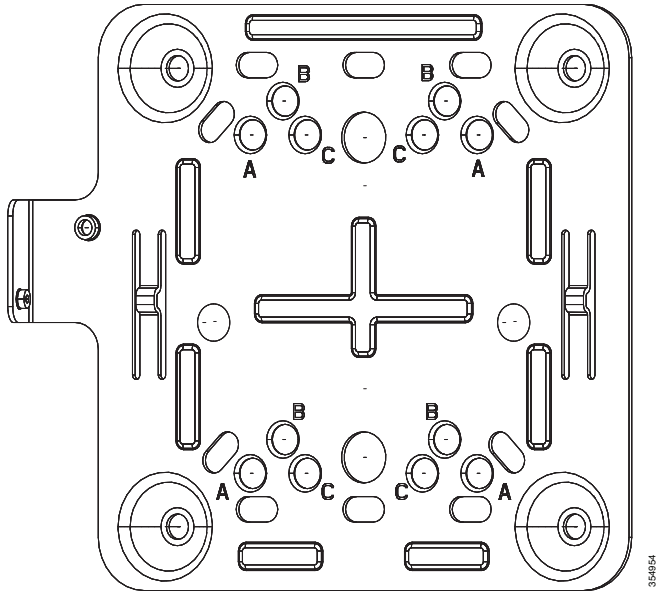
Figure 3 AIR-AP-BRACKET-8
