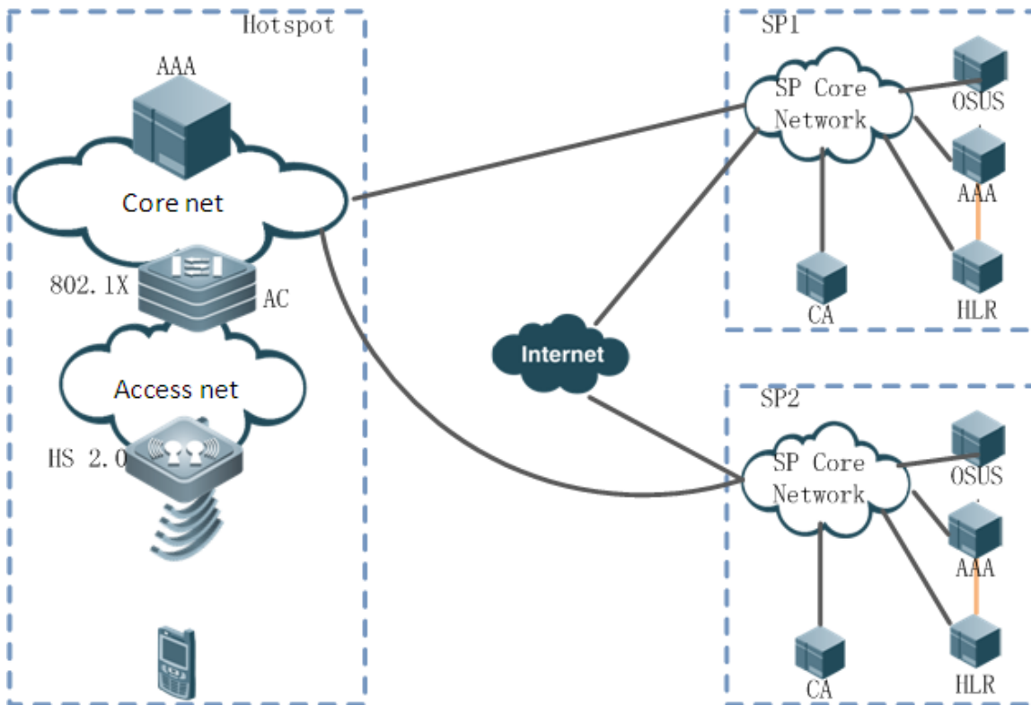
Figure 1-6 Structure of a Hotspot 2.0 Network
