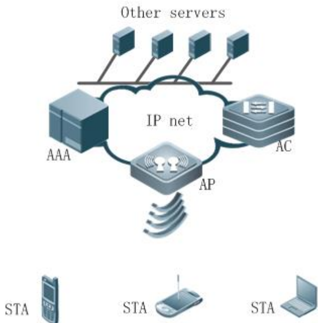
Figure 1-1 Topology of a Self-Built Hotspot 2.0 Network
