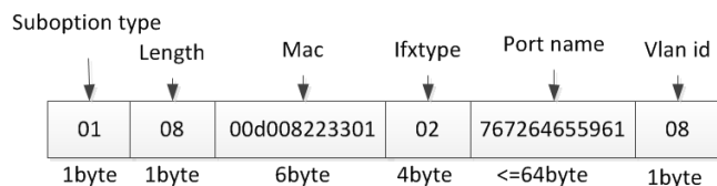
Figure 1-9 Option 82-remote-id
