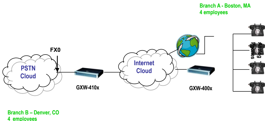
FIGURE 4: GXW400X & GXW410X SCENARIO/TOLL- FREE CALLING BETWEEN LOCATIONS
